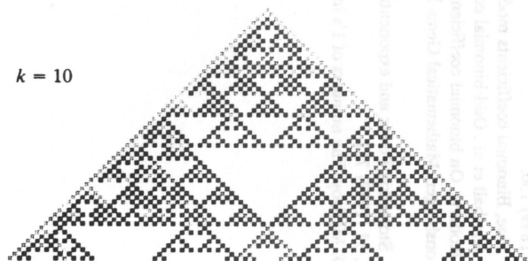
FIG. 4. Patterns obtained by reducing Pascal's triangle modulo k for several values of k . White squares indicate zeroes; progressively blacker squares indicate increasing values, up to k - 1 .
