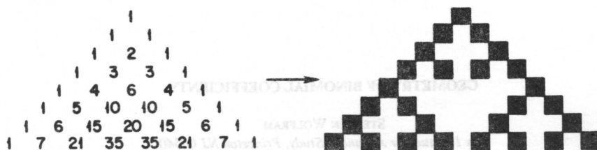
FIG. 1. The first few lines of Pascal's triangle modulo two.
